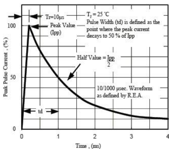
Fig. 5 - Pulse Waveform
